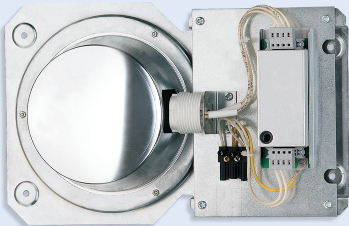
Image: Ceiling fitting light, round shaped 00 92 50 back view
