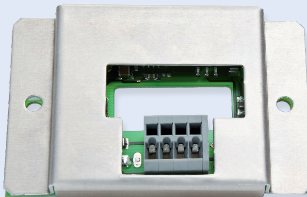
Image: Constant current supply for LED-modules A 80 250 700
