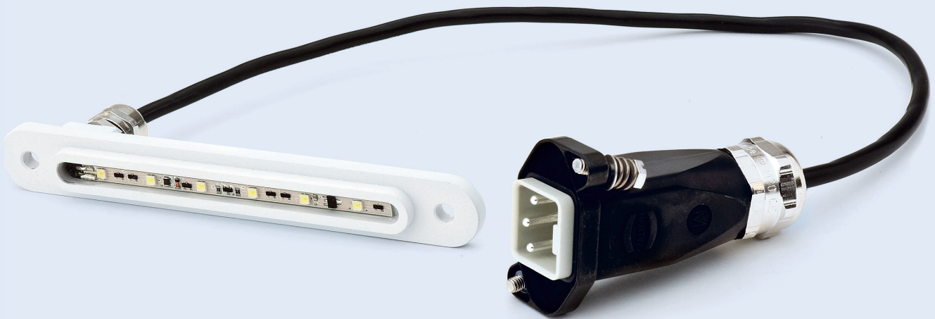
Image: LED exterior light/emergency light 143 538_08 with Harting plug in
